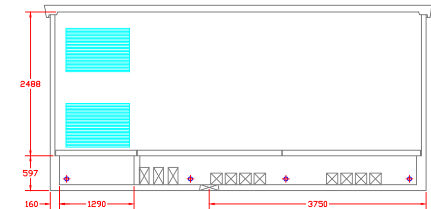
ALZADO PRINCIPAL
