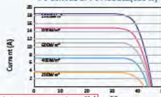
P-V CURVES OF PV MODULE(650W)
